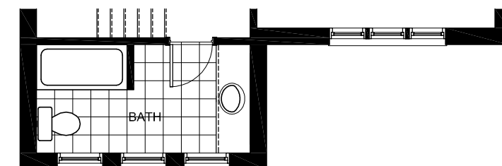
Partial Second Floor Plan - Elevation B
